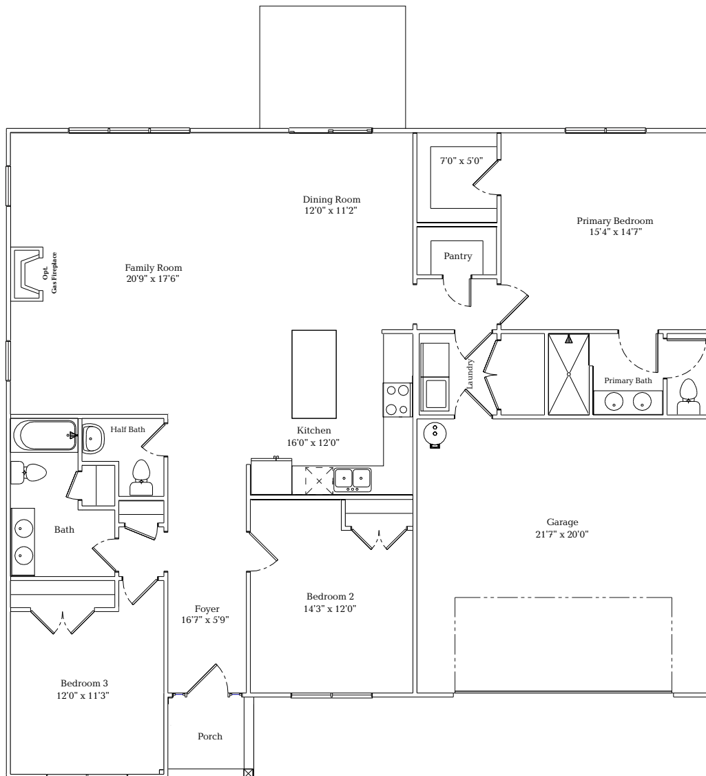
Standard First Floor
