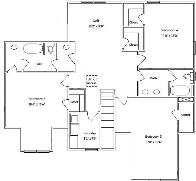
Standard Second Floor with finished Bedroom 2 and additional bathroom
