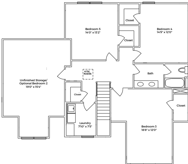
Standard Second Floor with finished Bedroom 5
