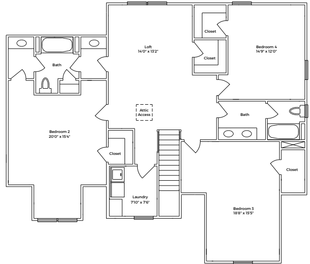
Second Floor with 4 foot bumpout- Finished Bedroom 2 with additional bathroom
